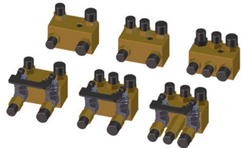
UCW-0475-59-00-00-0 Precise Machine Torch Holder Ø 30 mm (1.18")
