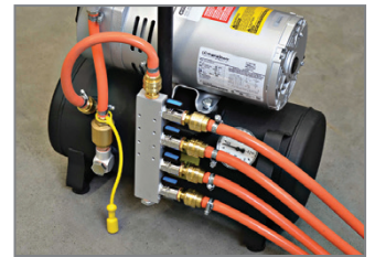
4-way manifold with connection cable • can separately connect vacuum units of up to four rails • allows rail leapfrogging during operation • ROZ-0541-04-00-00-0
